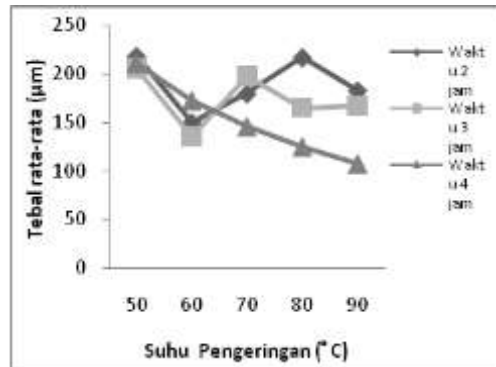
Gambar 3. Ketebalan ( \mu\text{m} ) plastik biodegradable
